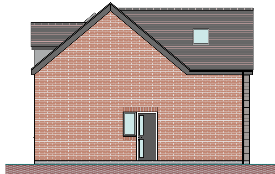
LEFT (EAST) ELEVATION SCALE 1:100
