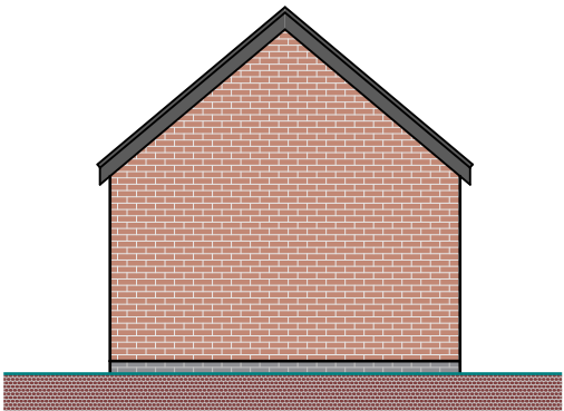
REAR (SOUTH) ELEVATION SCALE 1:100
