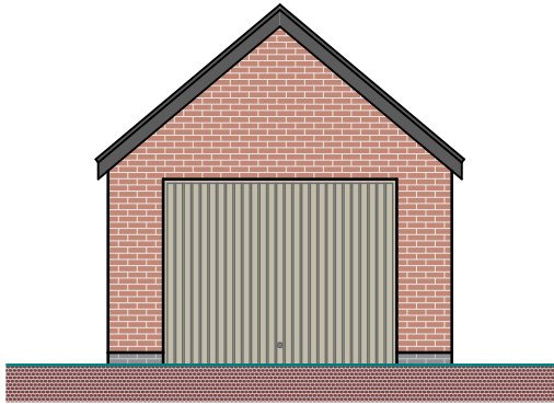
FRONT (NORTH) ELEVATION SCALE 1:100
