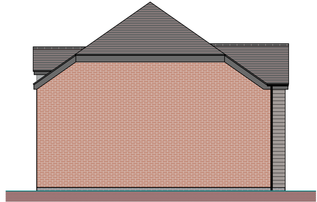
LEFT (EAST) ELEVATION SCALE 1:100
