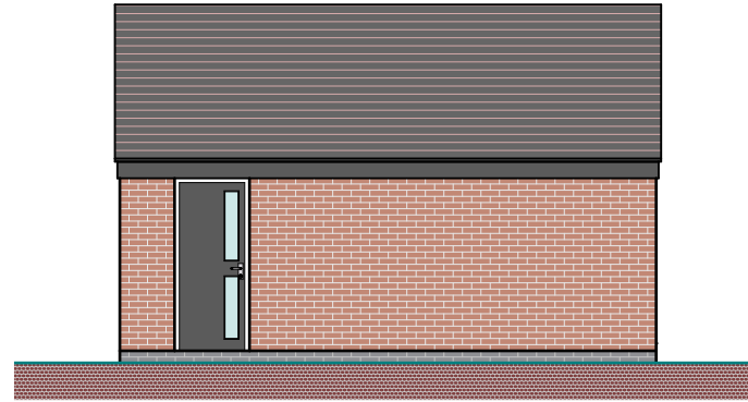
LEFT (EAST) ELEVATION SCALE 1:100
