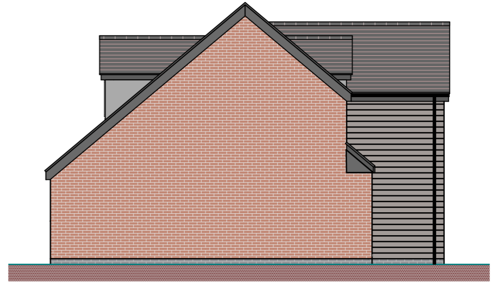
LEFT (NORTH) ELEVATION SCALE 1:100
